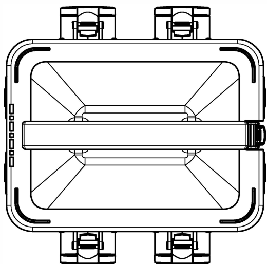
Figure 1 the construction of 2360-180 distribution box
