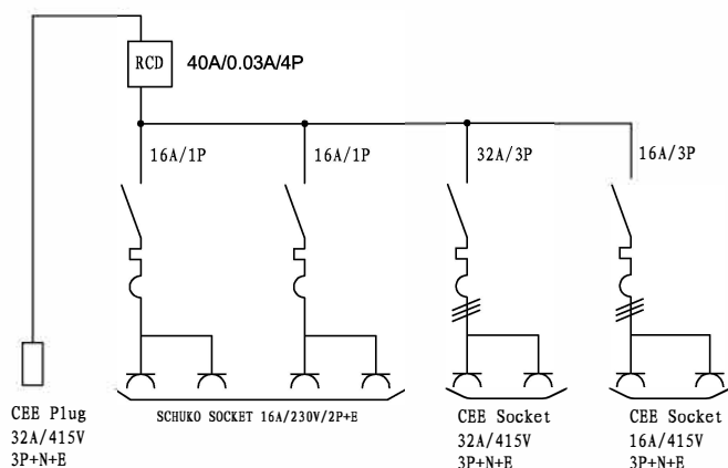
Figure 2 2360-180 assembly configure of electrical principle
